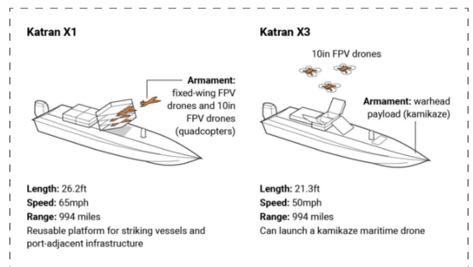
Katran X1 And Katran X3 Naval Drones. Source: United24
