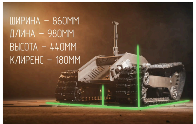
The "Strannik" V2. Source: The Defender
