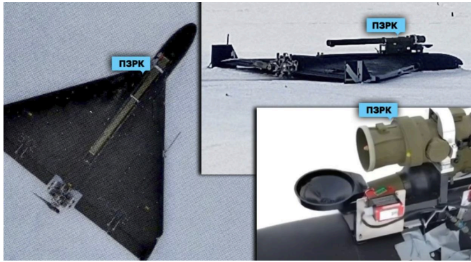
Figure 38. Serhii Beskrestnov (Flash). Russian Shahed UAV equipped with a MANPADS (Geran-4) 71.
