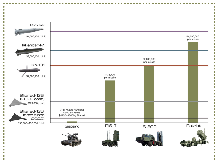
Figure 53. Cost-effectiveness comparison of intercepting Shahed-class UAVs and Kh-101, Iskander-M, and Kinzhal missiles using Gepard anti-aircraft gun systems and IRIS-T, S-300, and Patriot surface-to-air missiles.
