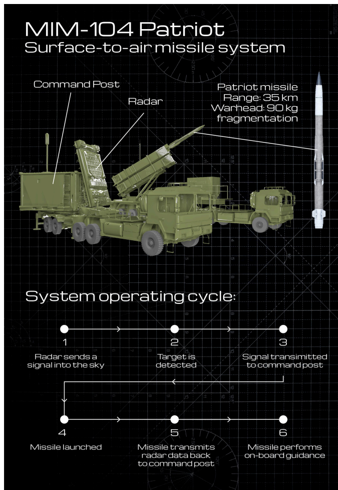
Figure 55. Fakty. How the Patriot air defense system works 110.
