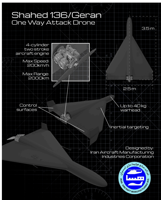
Figure 11. Wikipedia. Shahed-136.
